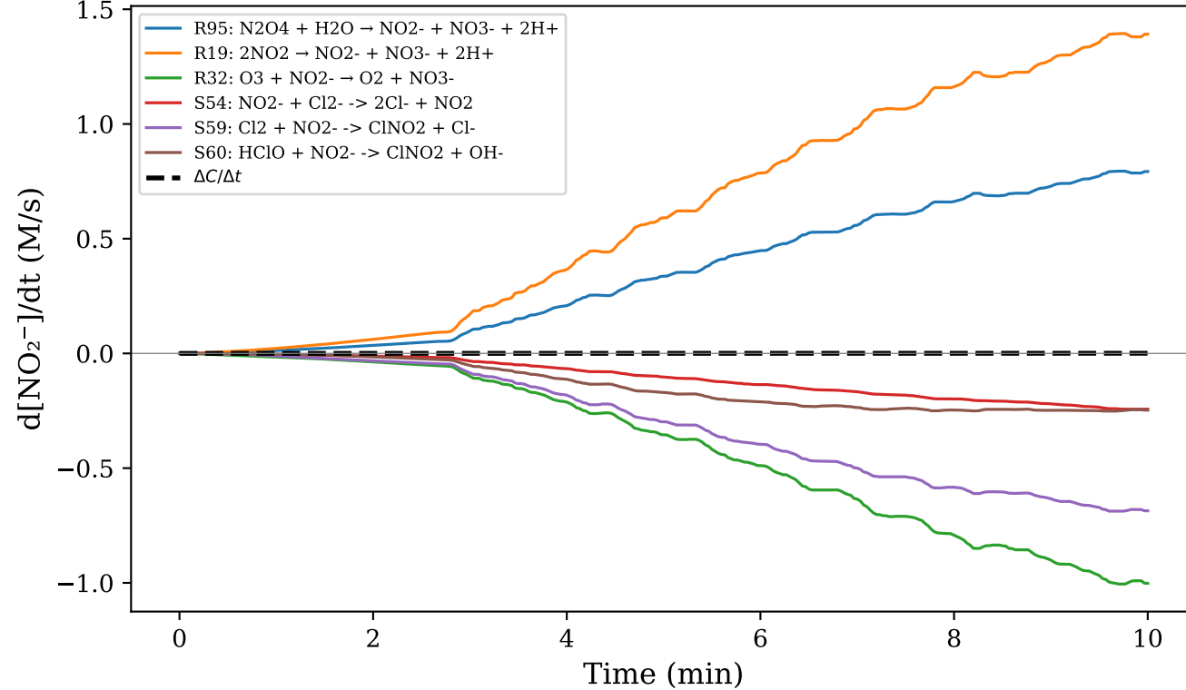
(c) \text{NO}_2^-
